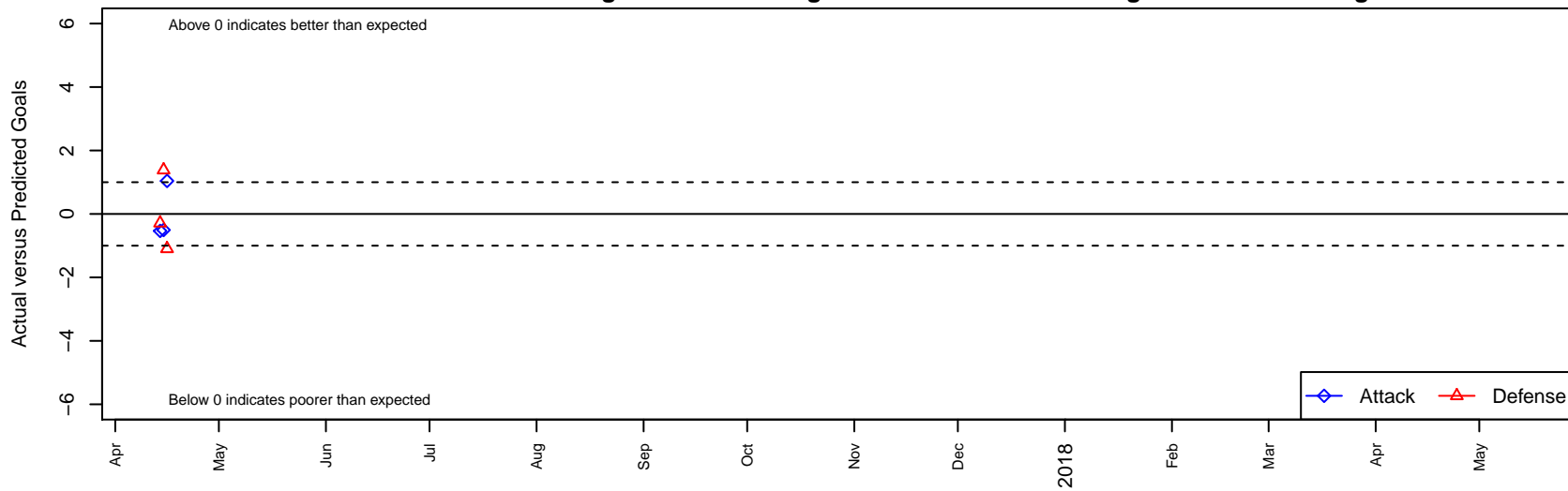
Coquitlam Metro Ford Porto B99 Dots are actual minus expected GF (blue circles) and GA (red triangles). Blue line is smoothed change in attack strength. Red is smoothed change in defense strength.
